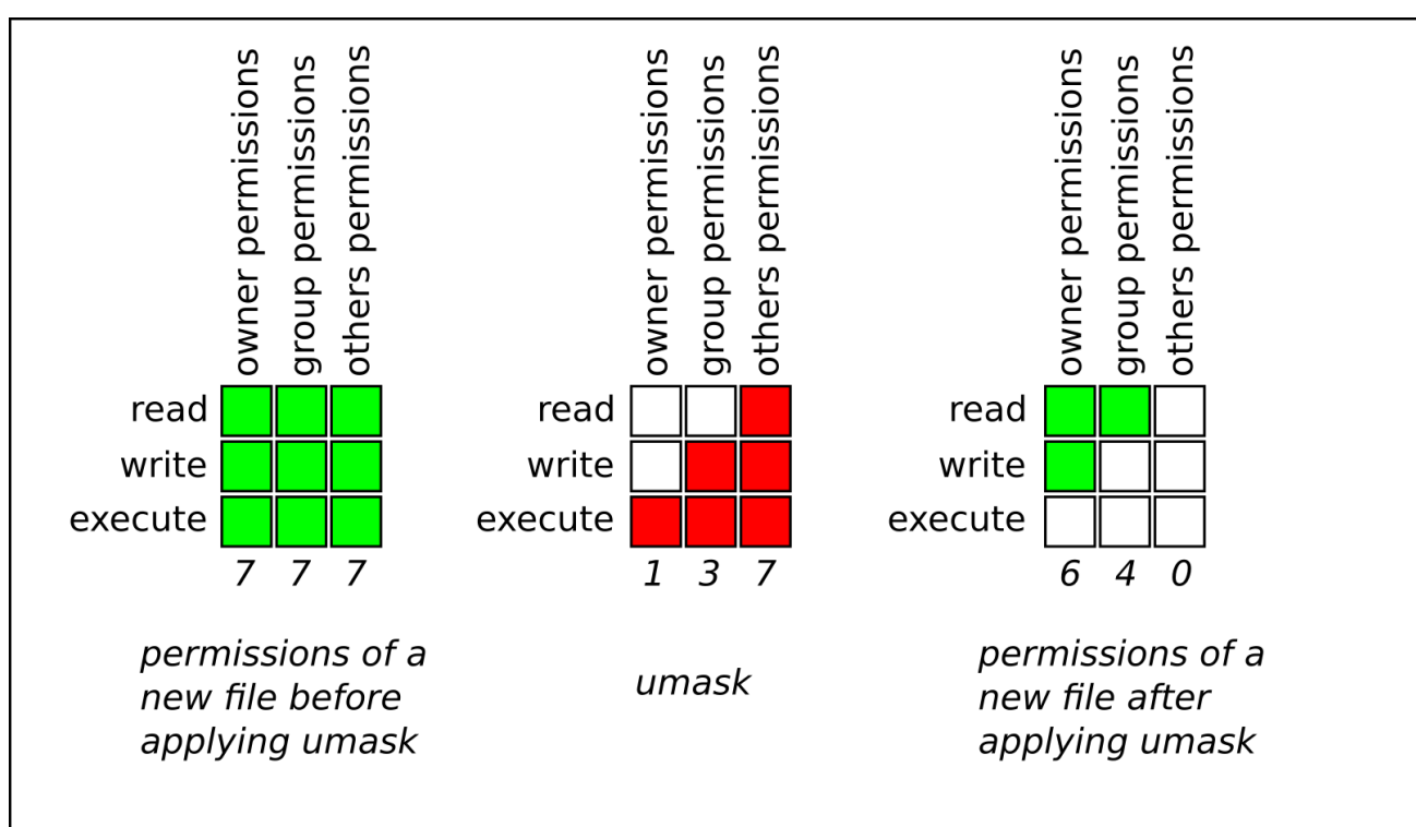
Figure 4.3. Applying umask when creating a file
